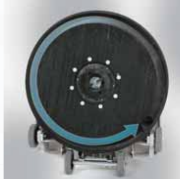
CM1500V with suction system. Through the spinning of the pad, a passive vac system channels the fine dust to a paper collection bag
