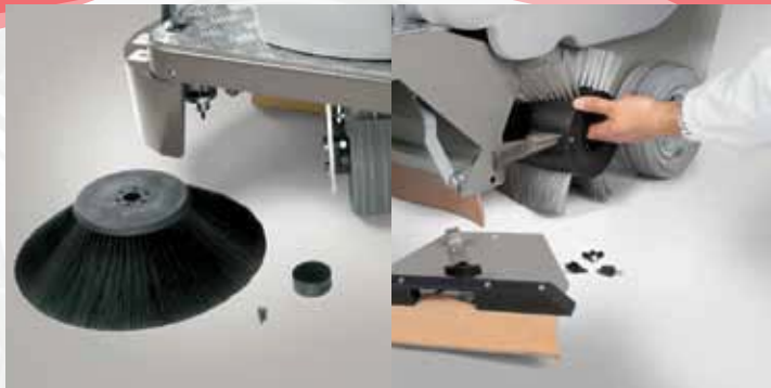
The side and central brush can be easily replaced without any tools
